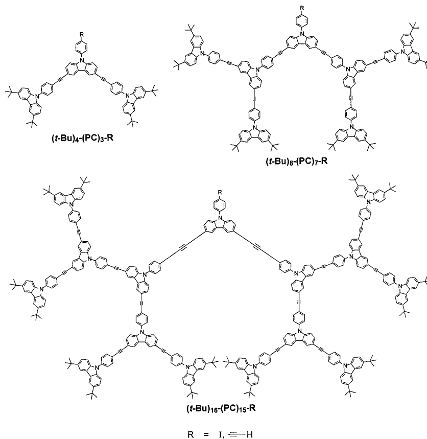
Figure 1. 9-Phenylcarbazole monodendrons with tert -butyl groups at the periphery.
