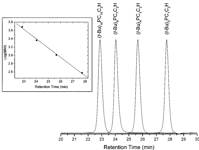
Figure 3. Normalized GPC chromatograms of 9-phenylcarbazole monomer and monodendrons bearing terminal acetylene focal points. The inset shows the linear correlation between the log of theoretical molecular weights and retention time [ \log(\text{MW}) = -0.22 \cdot t + 8.78 , R = 0.998 ].
